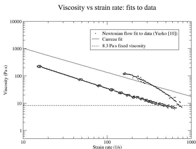
Fig. 6 : Viscosity laws for A357 at 0.49 fraction solid used to generate height vs. time data of Fig. 5
