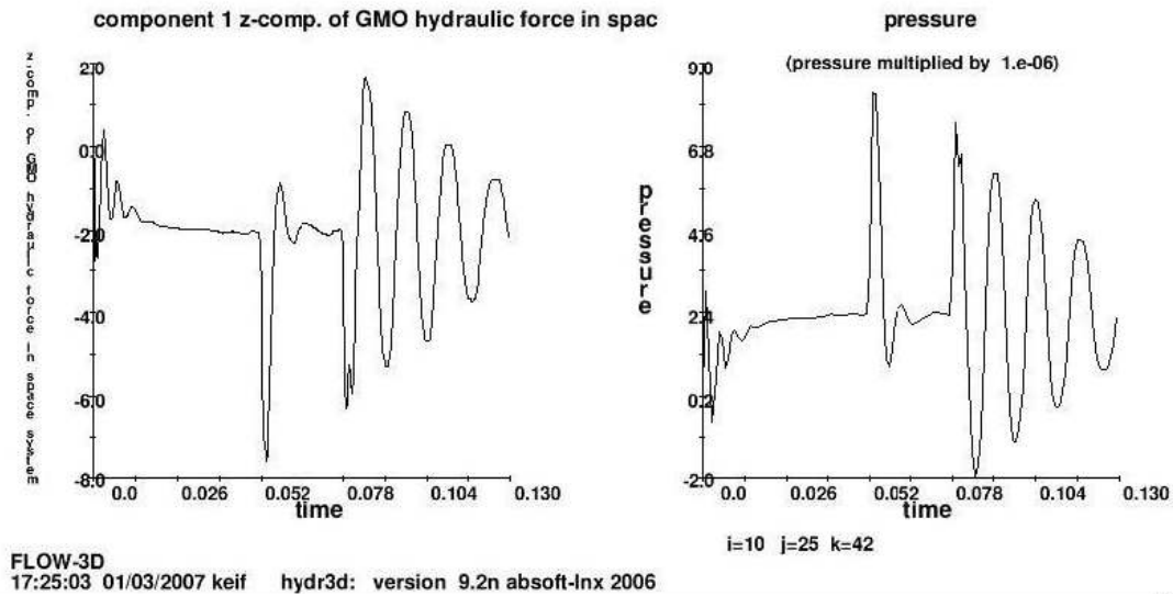
Fig. 2 : Hydraulic force on the plunger and a cavity pressure trace
