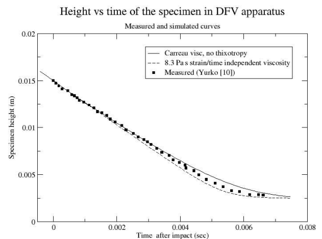
Fig. 5 : Sample height vs. time in one drop forge experiment and two simulated dependencies with different assumed A357 viscosity laws
