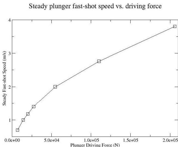
Fig. 4 : Simulation values for fast-shot speeds vs. plunger driving force
