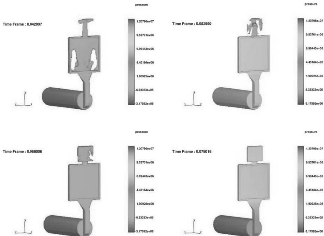
Fig. 3 : Filling patterns colored by pressure at 42 (top left), 53 (top right), 58 (bottom left) and 78 ms (bottom right)
