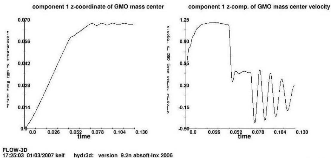
Fig. 1 : Plunger position and velocity vs. time for a typical fill simulation of a rimmed plate with a large back rim overflow.
